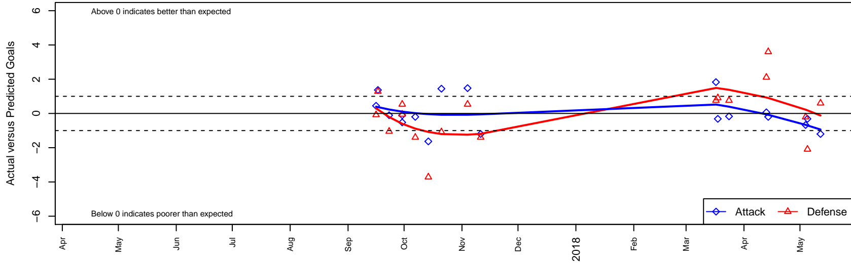
Spokane Foxes Tweedy G04 Dots are actual minus expected GF (blue circles) and GA (red triangles). Blue line is smoothed change in attack strength. Red is smoothed change in defense strength.
